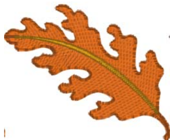
Gfe_pps_1_6.vp3
